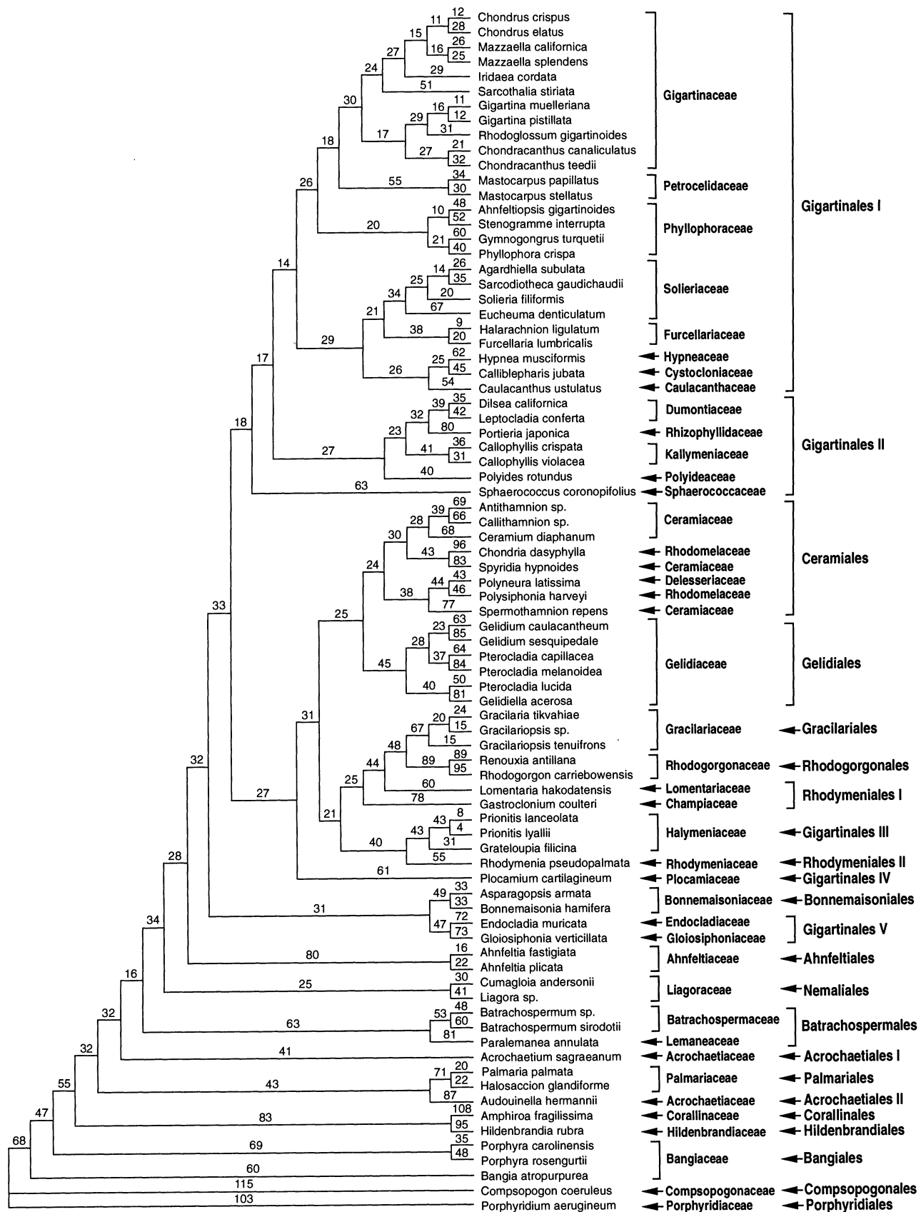
FIG. 1. Most parsimonious tree of rbcL from 81 red algal taxa of length = 6674, consistency index = 0.194, and retention index = 0.430. Branch length estimates are indicated above internodal branches.
